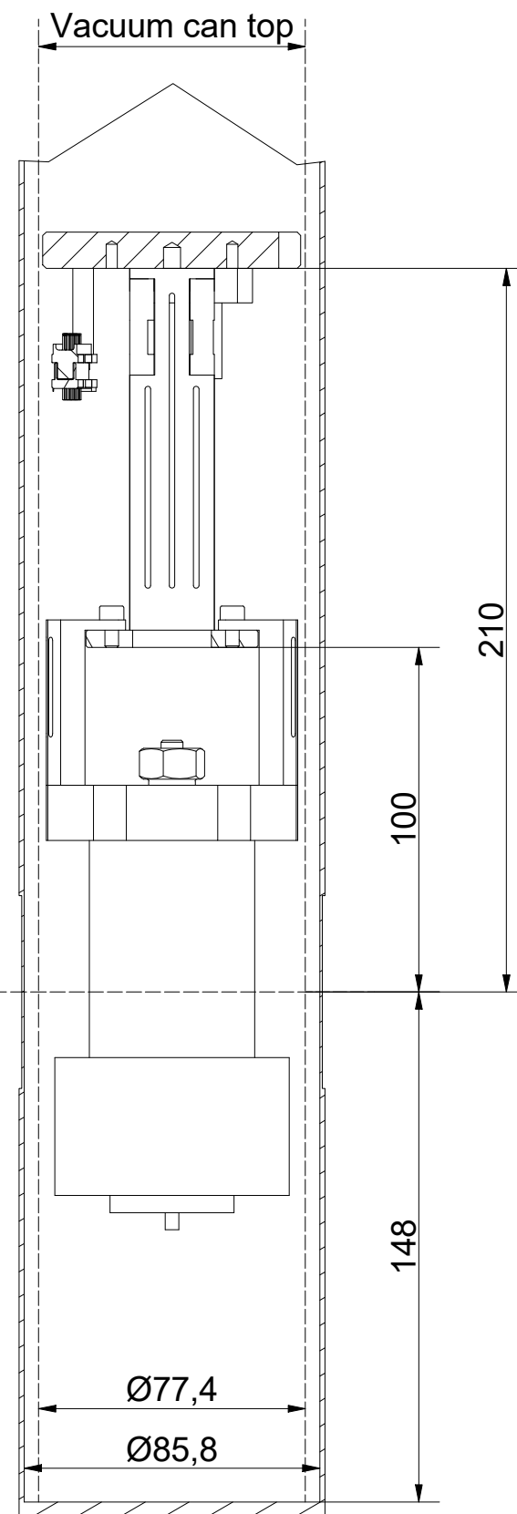
7kbar gas cell ( 1 : 2 )
